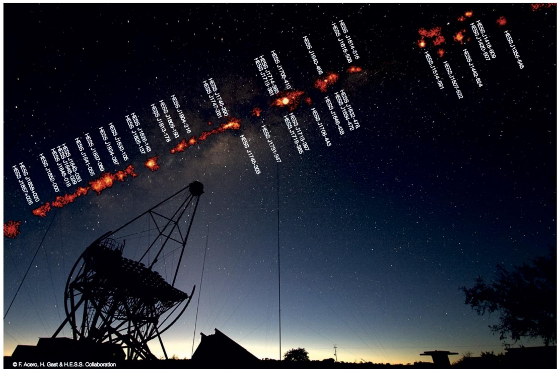
Montage showing very high energy gamma ray sources in the Milky Way, seen above the HESS telescopes in Namibia. (Photograph of the Milky Way seen above the HESS telescopes in Namibia: © F. Acero, / Map of gamma ray sources / © HESS collaboration)
